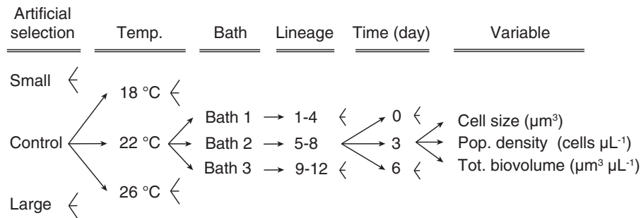
Figure 2. Experimental design. Three variables were monitored across a factorial design of three artificial selection treatments (i.e., small-selected, large-selected, and control), three temperatures (18, 22, and 26°C), three independent temperature baths, each containing four independent lineages that were monitored at day 0, 3, and 6 after inoculation (972 observations).
